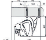
Top-fix
