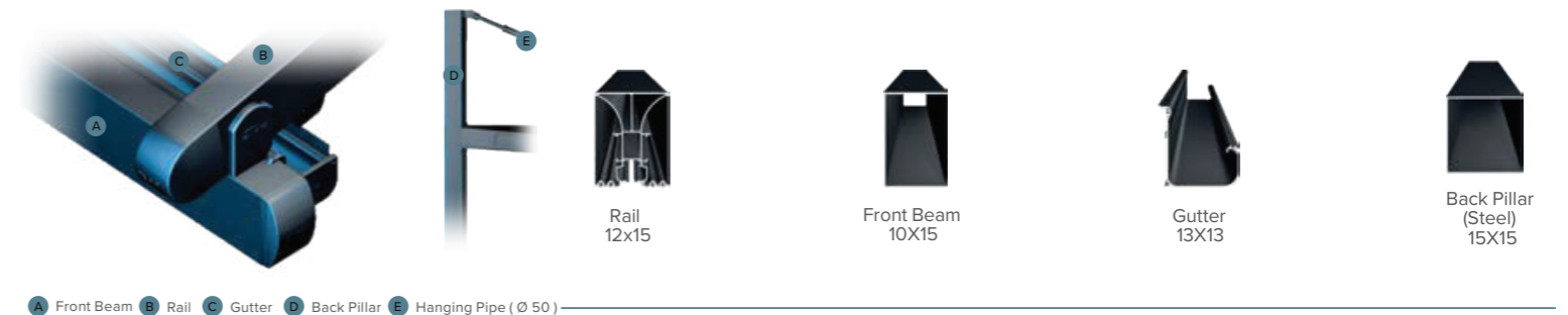
A Front Beam B Rail C Gutter D Back Pillar E Hanging Pipe (Ø 50)
